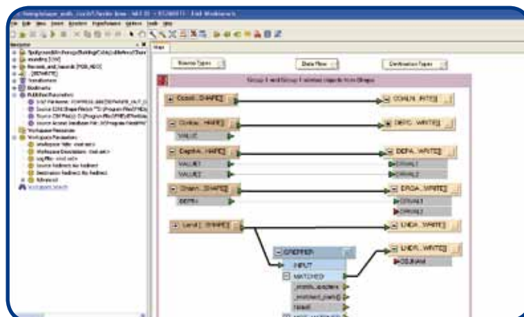
FME Workbench with S-57 Writer
